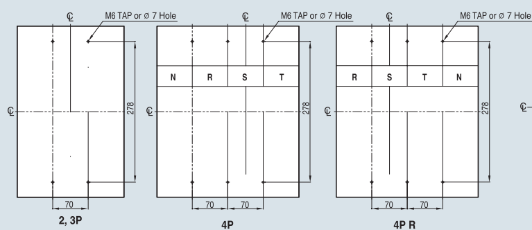
Panel drilling
